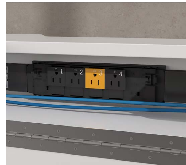
Hover offers an 8-wire/4-circuit system that is UL-listed. One circuit can be centrally controlled in accordance with CA Title 24 and other local regulations.
