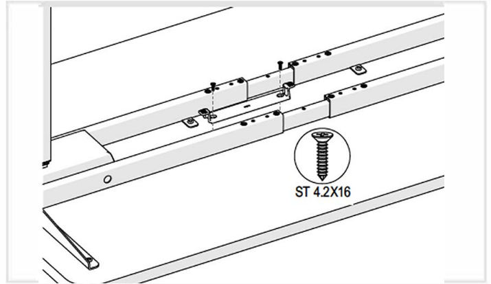
Step 8 Mount the Control Unit Bracket as illustrated above. Please refer to Torque Guide.
