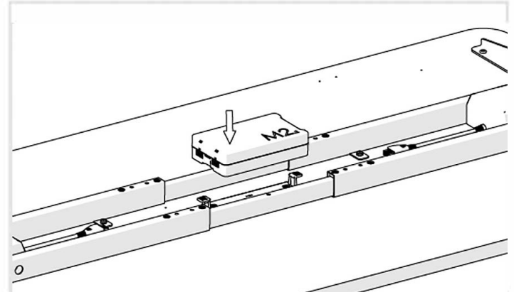
Step 10 Mount the Control Unit as illustrated above.
