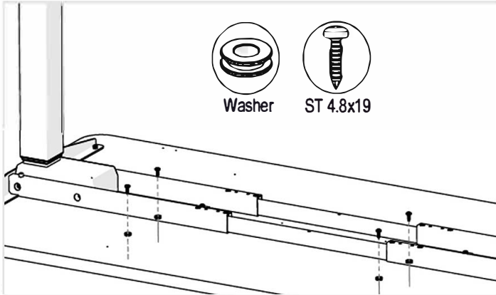
Step 7 Mount the Smart Tray Washers as illustrated above. Please refer to Torque Guide.
